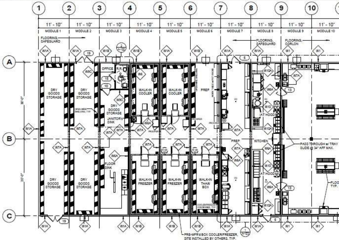
21-Box Dining Facility – Enlarged Kitchen Plan
