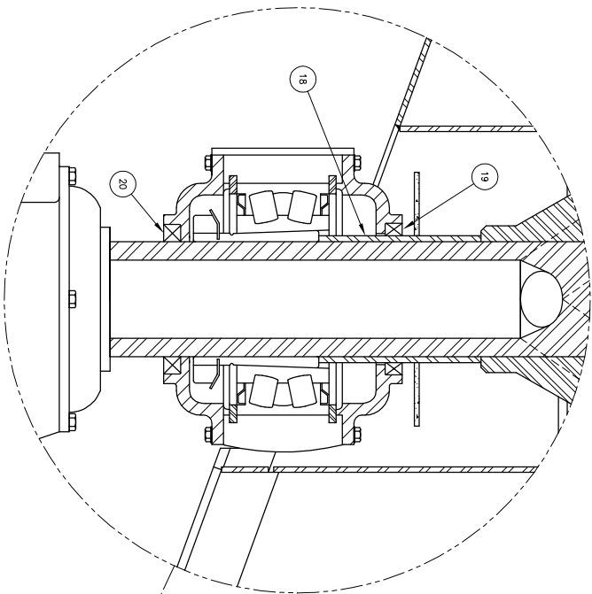
UPPER BEARING DETAIL
