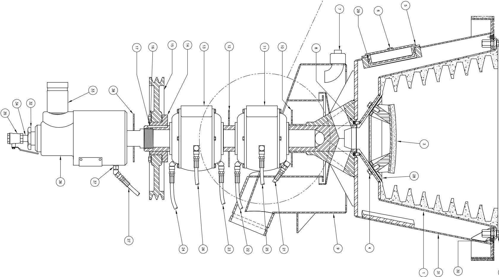
ROTOR ASSEMBLY
