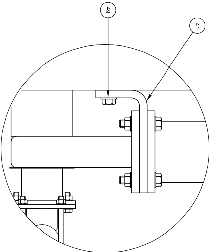
-SIDE VIEW DETAIL OF ICS MOUNT-
