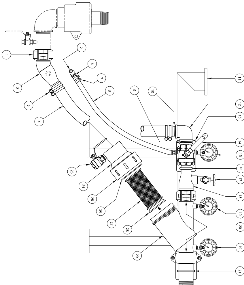
MODEL KC-CD20 MANUAL PIPING ASSEMBLY c/w FILTER
